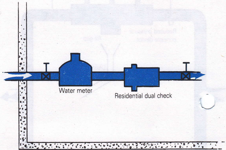
FIGURE 37 Typical Installation Residential Dual Check with Straight Set and Copperhorn
