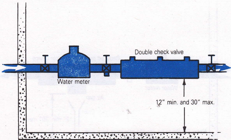
FIGURE 36 Typical Installation Double Check Valve Horizontal and Vertical Installation
